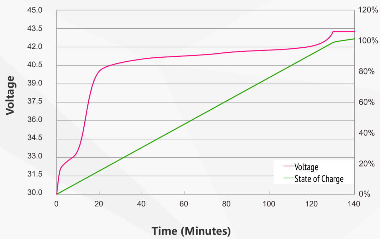
Charging Characteristics (0.5C @25°C)
