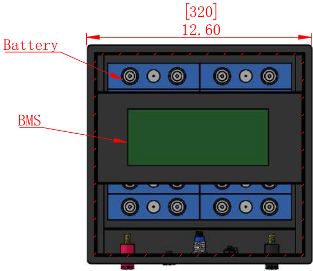
Section view A-A 1 : 5.5
