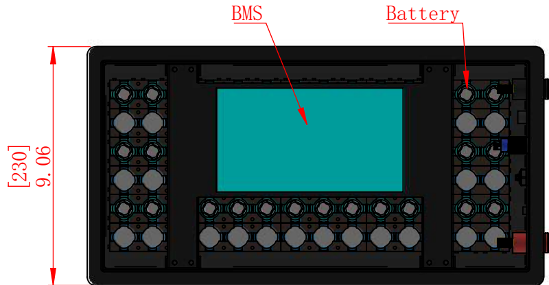
Section view A-A 1 : 5
