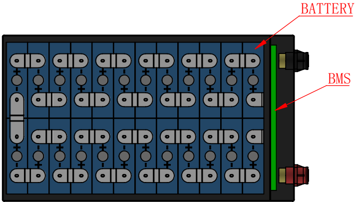
Section ViewA-A 1 : 6.5
