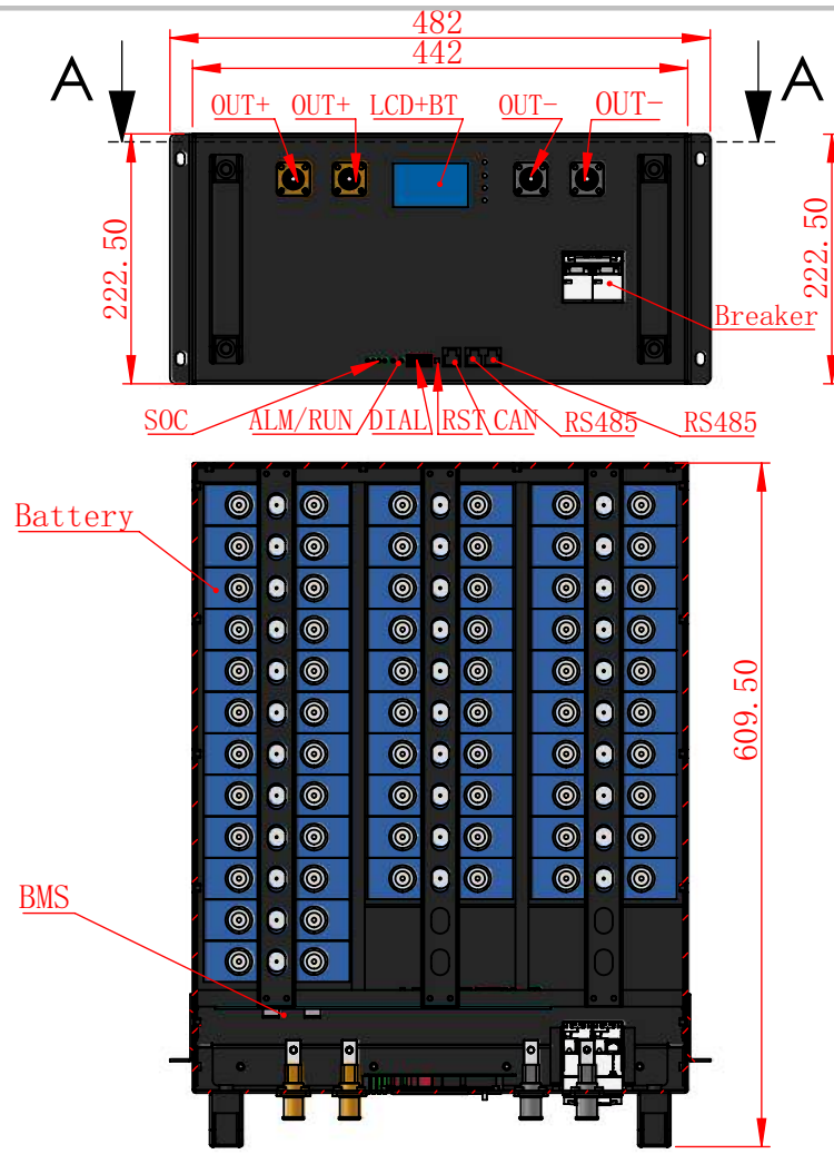
Section view A-A 1 : 7.5
